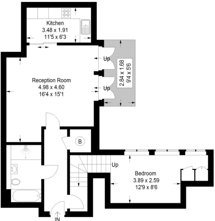
Fourth Floor
